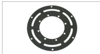
CWN-D213 衔铁片中间弹垫 φ120Xφ239X2.0 DORNIER
