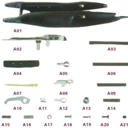
CWN-D007 多尼尔III送剑 (特种) Sending Gripper-Dornier III
