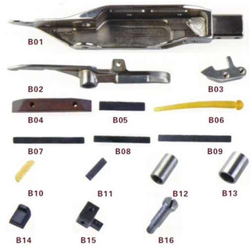
CWN-D004 多尼尔II接剑 Receiving Gripper-Dornier II
